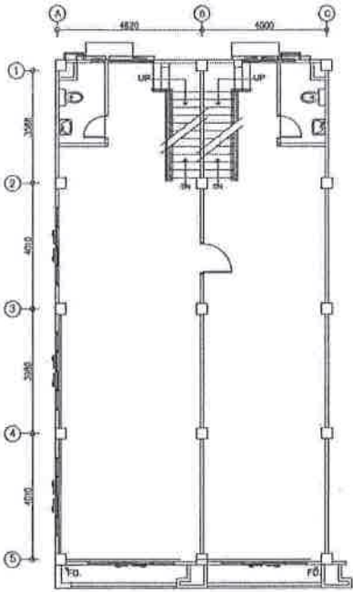
4th FLOOR PLAN 1:100
