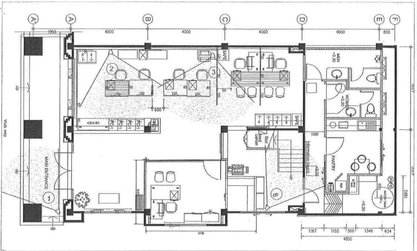
FIRST FLOOR EXIM BANK RAMA 2
