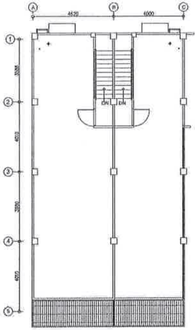
5th FLOOR PLAN 1:100
