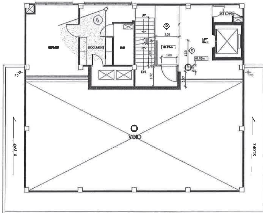
FURNITURE LAYOUT PLAN ( MEZZANINE FLOOR PLAN ) SCALE
